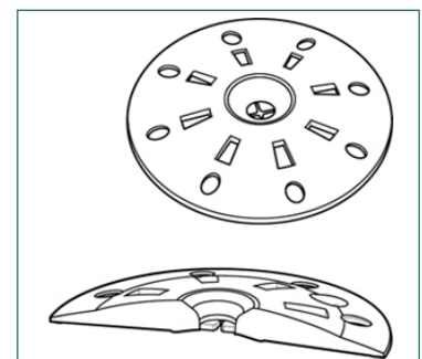
Section Detail: Cupped underside seals washer around membrane
